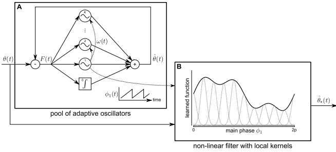
Fig. 1. Online learning of a periodic but non-sinusoidal input signal \theta(t) . A : pool of adaptive oscillators (1), (4), decomposing the input into a real-time Fourier series. B : kernel-based non-linear filter, mapping the phase of the main harmonic \phi_1(t) to the input envelope. Adapted from [18].
